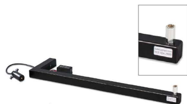
HMLA* Threaded Base, Includes 7-Way Plug and built-in 107db Backup Alarm (Non-powered, Part #: HMLNPA)
